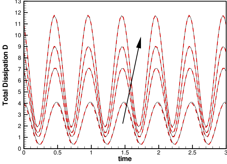
FIGURE 6. Total dissipation D(t) for \epsilon = 0.1 , N = 2 , and \mathbb{A} = -0.5 . Solid lines: numerical results; dashed lines: asymptotic predictions from (3.40). \alpha^2 = 10, 100, 200, 400 increasing in the direction of the arrow.
