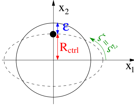
FIGURE 1. Sketch of the 2D problem for the transverse flows: The tube wall performs a high-frequency oscillation of amplitude \epsilon and induces an oscillatory flow. The radius R_{ctrl} of the control point on the wall is used to characterise the wall deformation. The Lagrangian coordinate \zeta = \xi^2 is used to parametrise the wall shape. The sketch illustrates the wall deformation for the N = 2 mode.
