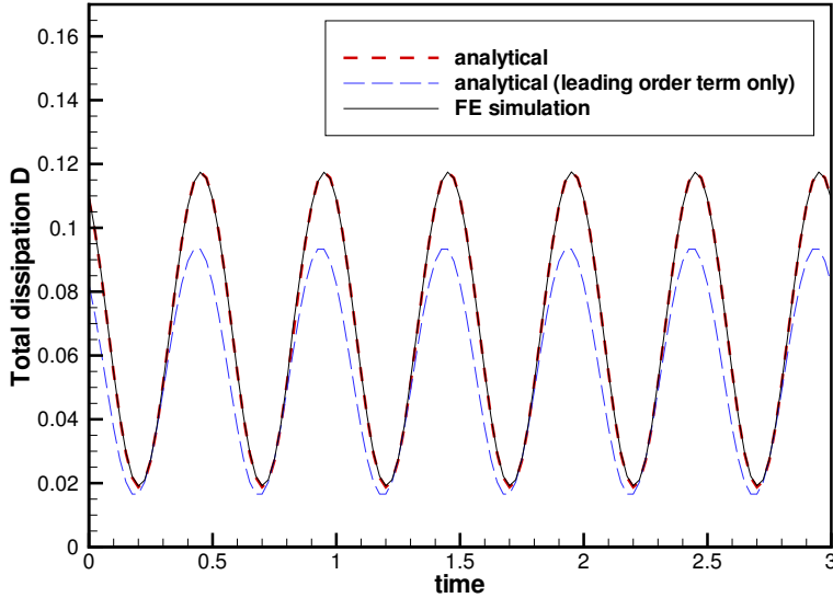
FIGURE 5. Total dissipation D(t) for \epsilon = 0.01 , N = 2 , \mathbb{A} = -0.5 and \alpha^2 = 400 . Solid lines: numerical results; broken lines: asymptotic predictions from (3.40).
