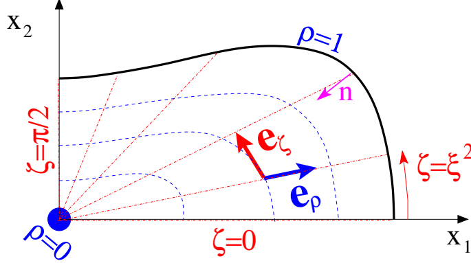
FIGURE 4. Sketch of the body-fitted coordinate system (\rho, \zeta) and the boundary-layer coordinate n .
