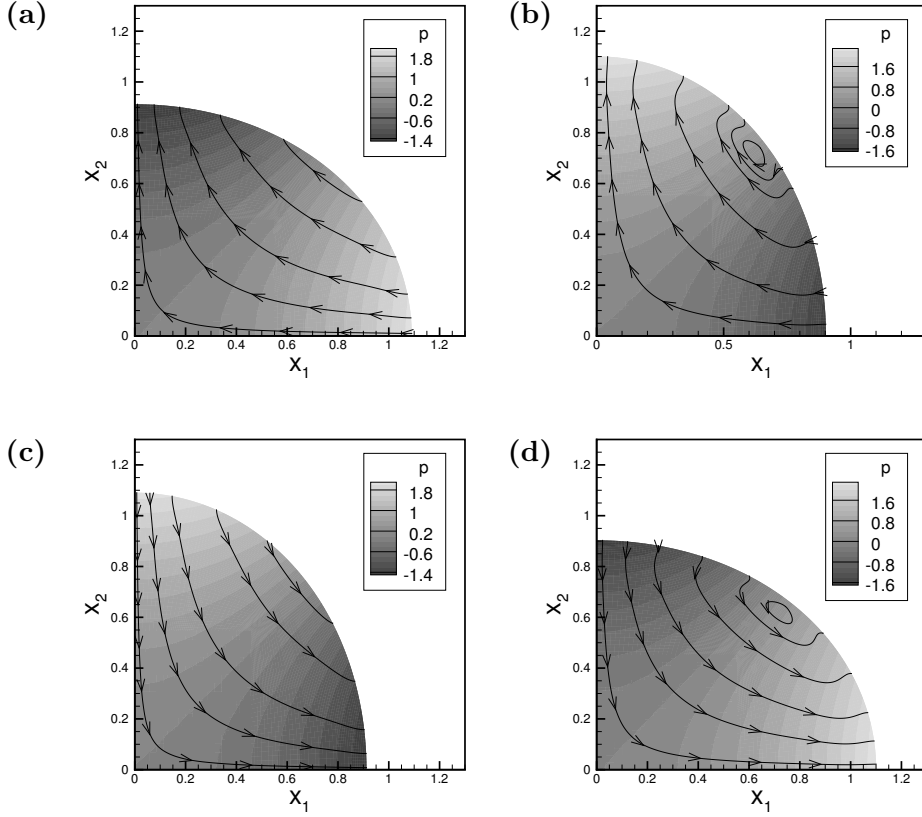
FIGURE 2. Streamlines and pressure contours during four instants of the oscillation. \alpha^2 = 100 , \epsilon = 0.1 ; wall motion given by (3.17) with N = 2 and \mathbb{A} = -0.5 . (a) t = 0.325 , (b) t = 0.725 , (c) t = 0.825 , (d) t = 1.225 . Only one quarter of the domain is shown.
