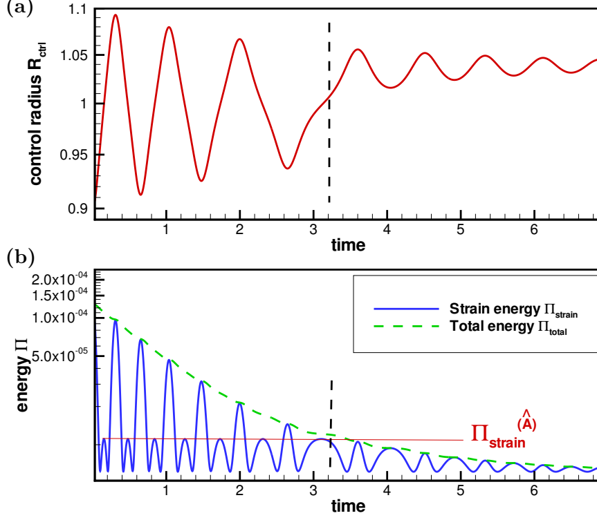
FIGURE 10. Illustration of the energy budget during the oscillation shown in Fig. 8(c). (a) shows the evolution of the control displacement; (b) shows the corresponding energies. The character of the oscillation changes when the system's total energy drops below the strain energy \Pi_{\text{strain}}^{(\hat{A})} required to traverse the approximately axisymmetric configuration.
