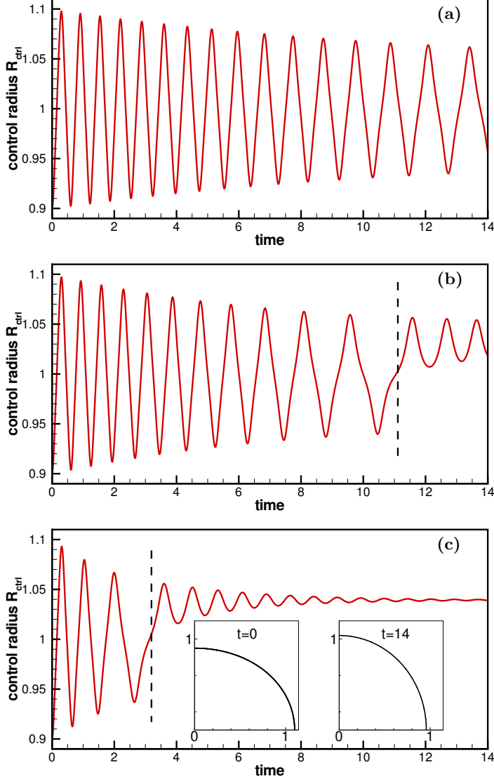
FIGURE 8. Time-trace of the control radius R_{ctrl}(t) for oscillations with fluid-structure interaction for \rho_w/\rho_f = 0 and h/a = 1/20 . Initially, the fluid and the wall are at rest and the initial wall displacement field is given by (3.18) with N = 2 , \mathbb{A} = -0.5 and an amplitude of \epsilon = 0.1 . (a) \alpha^2 = 100 ; (b) \alpha^2 = 50 ; (c) \alpha^2 = 10 . The dashed vertical lines indicate the transition from type I to type II oscillations. The two insets in (c) show the initial and equilibrium wall shapes for \alpha^2 = 10 .
